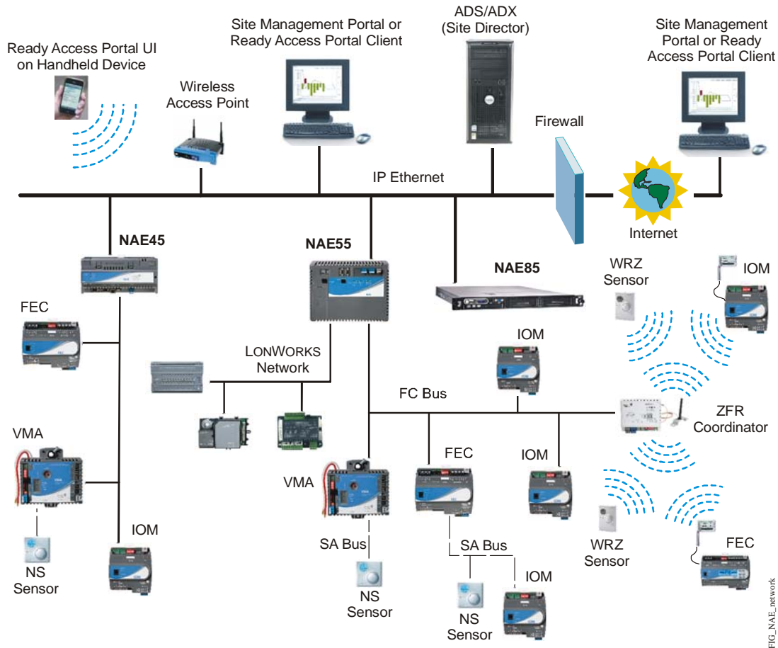
Figure 1: Diagram of Metasys Network with NAEs
